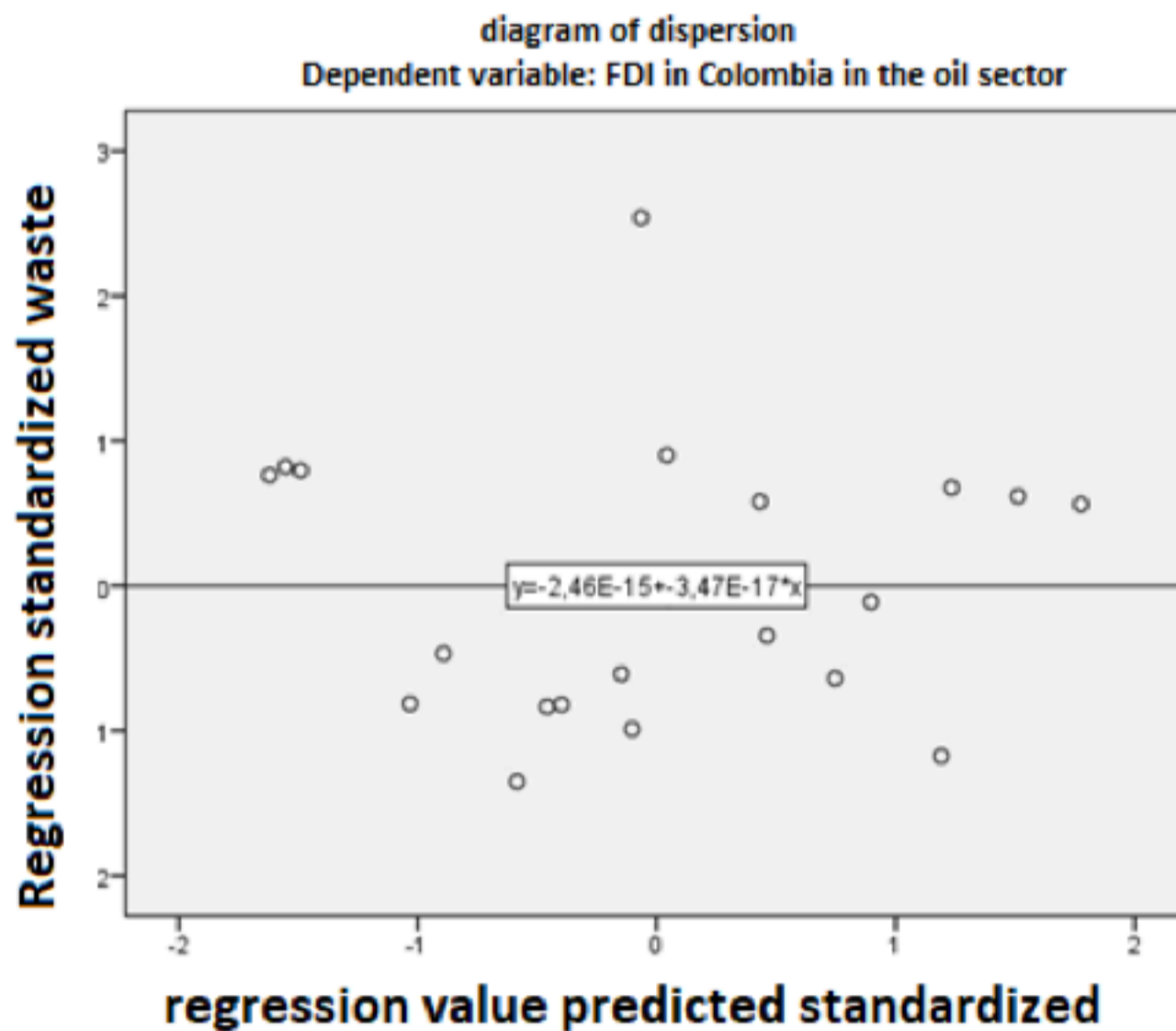
Figure 3 Homocedasticity test
